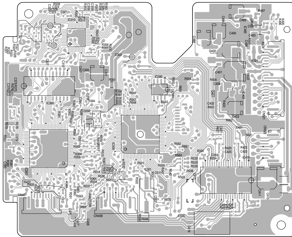
(Servo board)
