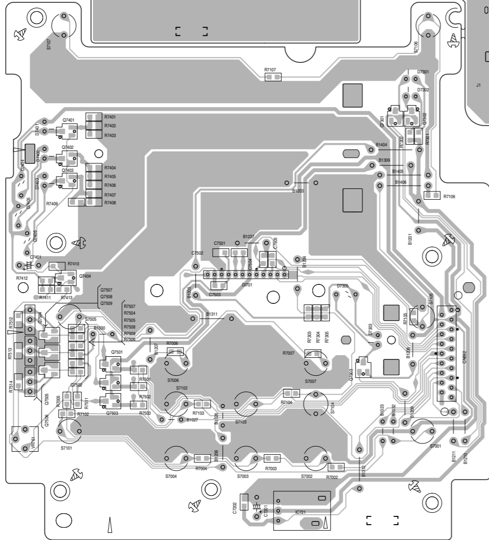
(Front board)
